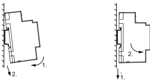
Figure 1: Mounting
