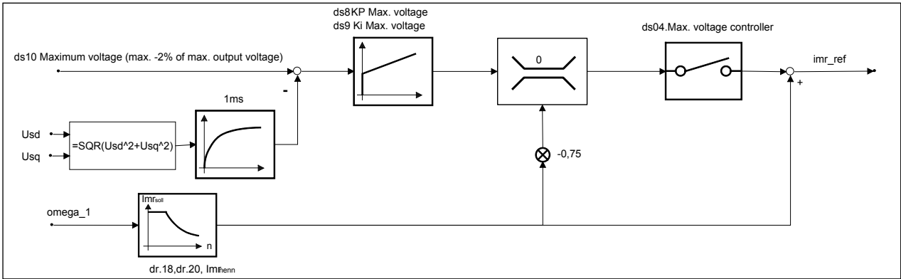
Figure 7.5.3.d Field weakening
