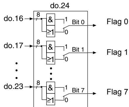
Figure 7.3.20 Linking the switching conditions in logic step 1
