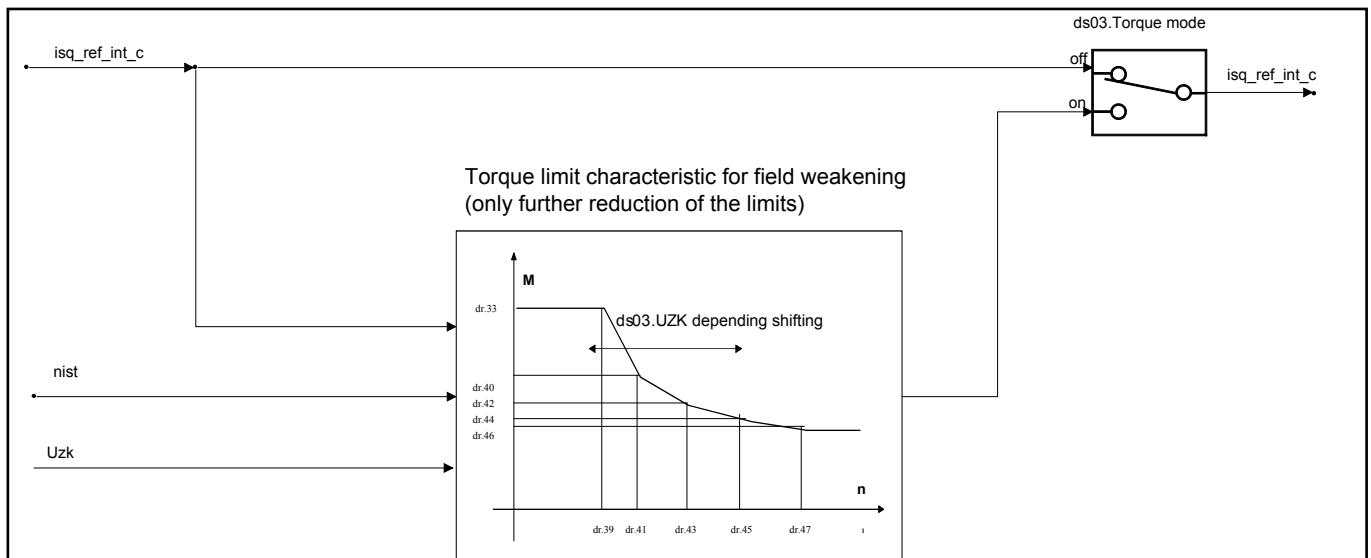
Figure 7.6.4.d Field weakening
