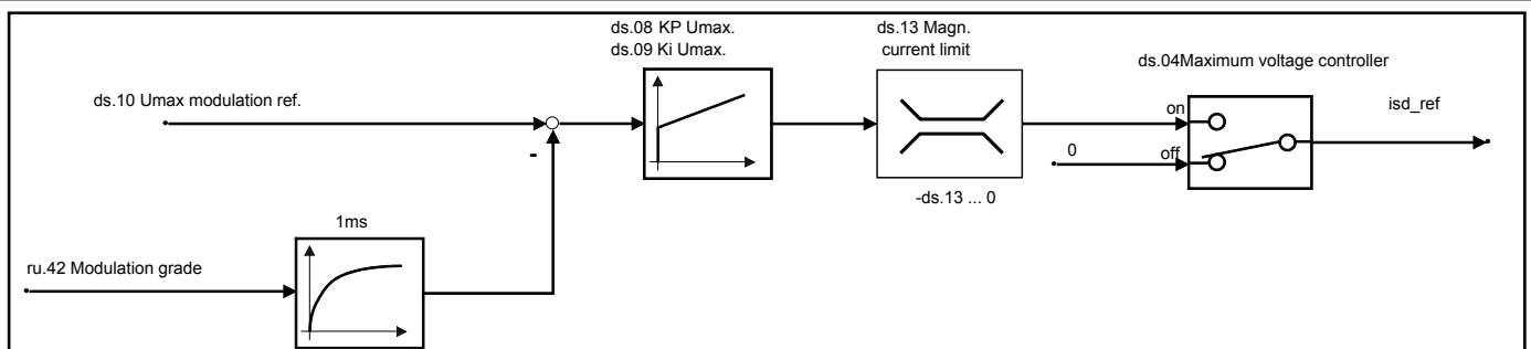
Figure 7.6.4.d Field weakening
