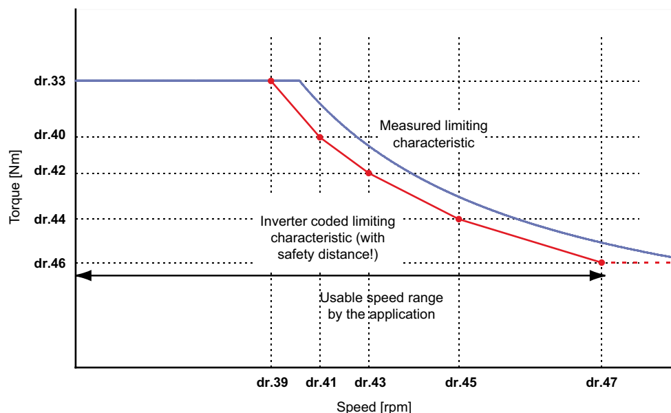
Figure 7.8.3.2.2 Limiting characteristic
