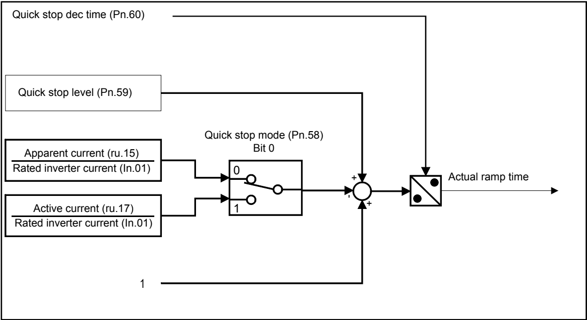
Block diagram of the differential control:
