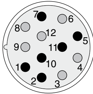
Fig. 7.11.2.b Resolver connector at the KEB servo motor
