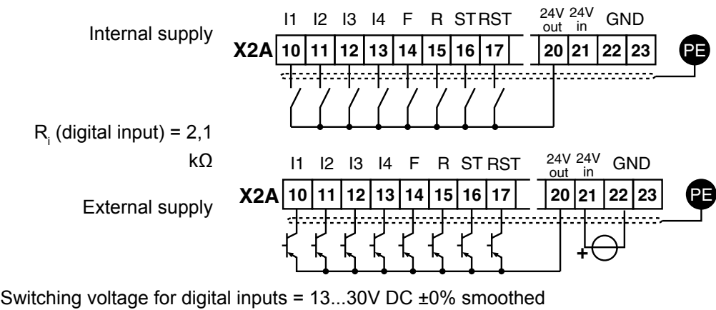
Figure 7.3.2.a Digital inputs in PNP control (di.00 = 0)
