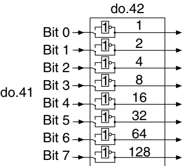
Figure 7.3.23b. Inversion of Outputs
