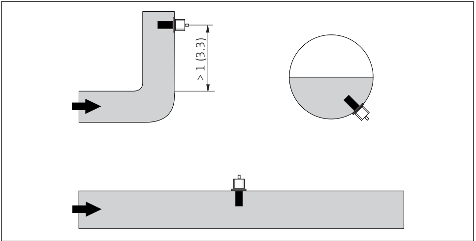
4 Installation positions of the conductivity sensor
