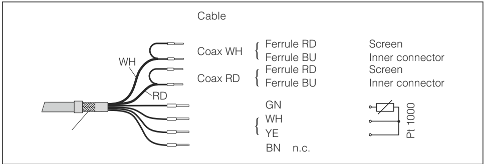
8 Fixed cable / measuring cable CLK6
